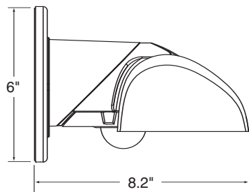
Wall-Mounted Configuration
