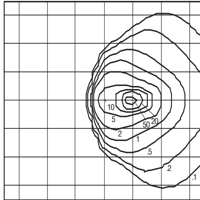
GP2 Spot Optics 175w Metal Halide Mounting Height: 15 ft. - Tilt: 45° Lumens: 14000 NEMA: 2H x 3V
