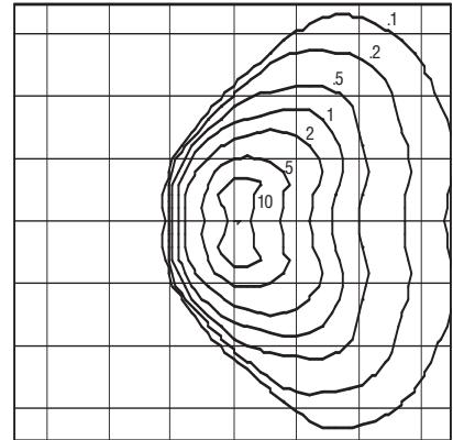
GP2 General Purpose Optics 175w Metal Halide Mounting Height: 15 ft. - 30° Lumens: 14000 NEMA: 7H x 7V
