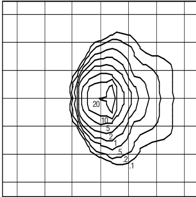
GP2 Cutoff Optics 175w Metal Halide Mounting Height: 15 ft. - Tilt: 30° Lumens: 14000 NEMA: 6H x 5V
